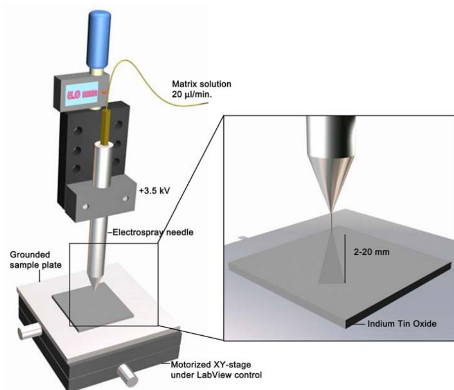
Figure 3. Schematic representation of the electrospray set-up.
