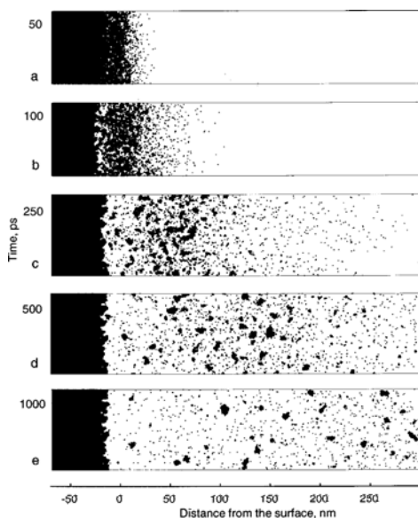
Figure 2. Time development of the MALDI plume in a 2D simulation. The total fluence is approximately twice the threshold fluence for ablation. Taken from reference 112
