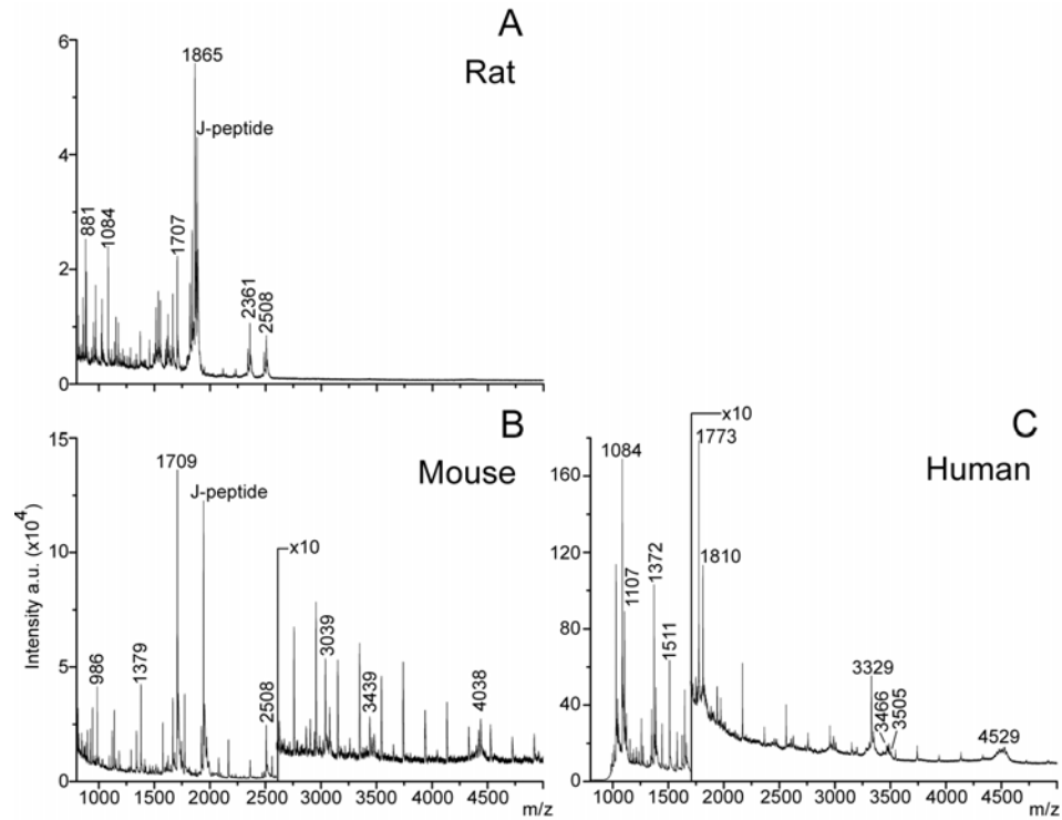
Figure 2. MALDI-IMS spectra of mammalian pituitary tissue sections. Summed mass spectra of direct MALDI analysis of a (A) HCCA covered rat pituitary, (B) DHB covered mouse pituitary and (C) HCCA covered human pituitary tissue section.
