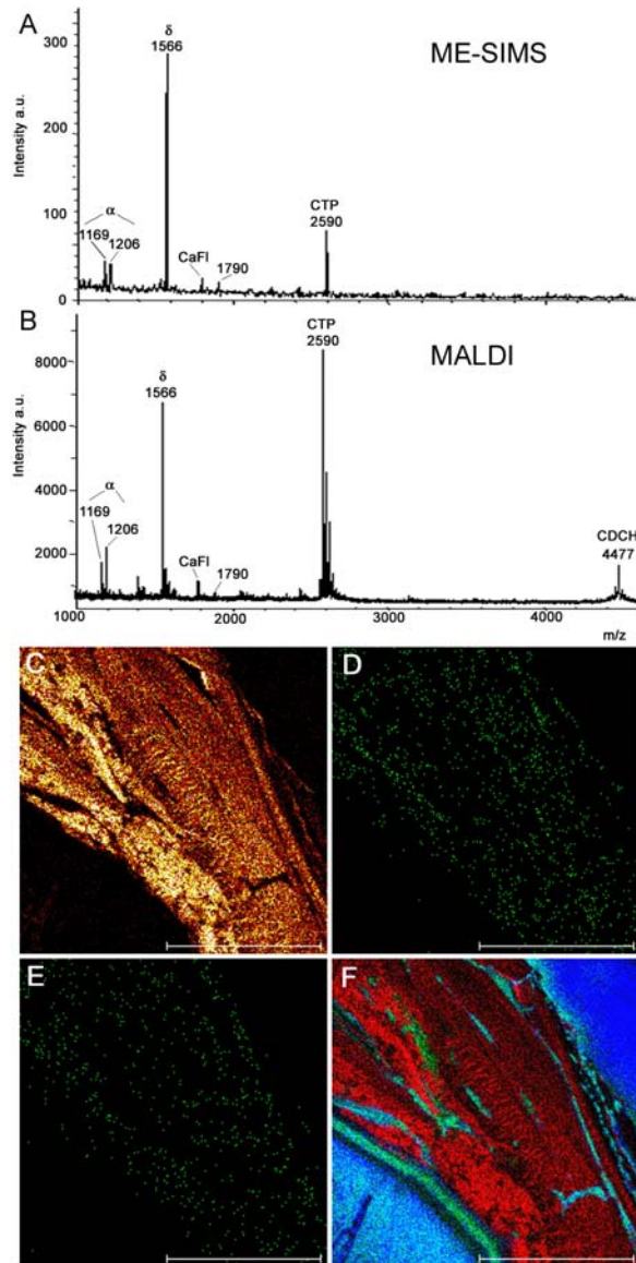
Figure 2. ME-SIMS vs. MALDI. (A) ME-SIMS and (B) MALDI spectrum of a commissure extract of the pond snail Lymnaea stagnalis . Both spectra were obtained using standard dried droplet sample preparation with DHB as matrix. The peptides identified are; \alpha -caudorsal cell peptide ( \alpha , protonated and cationized), \delta peptide ( \delta ), HFFYGPYDVFQRD Vamide ( m/z 1790), Calfluxin (CaFI), carboxyl terminal peptide (CTP) and caudodorsal cell hormone (CDCH). The ME-SIMS measurements used indium primary ions (total ion dose 8.9 \times 10^{11} ions/cm 2 ) and the MALDI experiments 250 shots of the 4 ns 337 nm nitrogen laser.
