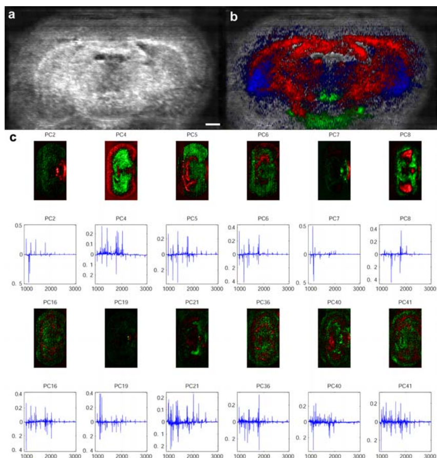
Figure 4. Example of images obtained with microscope MALDI-IMS. (a) High-resolution microscope mode TIC image of a rat brain tissue section. (b) The same microscope mode TIC image with overlain microprobe m/z data (m/z 1085 (vasopressin) in green, m/z 2030 in red and m/z 1431 in blue). (c) Correlation between different m/z species found in the microprobe dataset of the rat brain tissue section by PCA analysis. (Scale bar is 1 mm).
