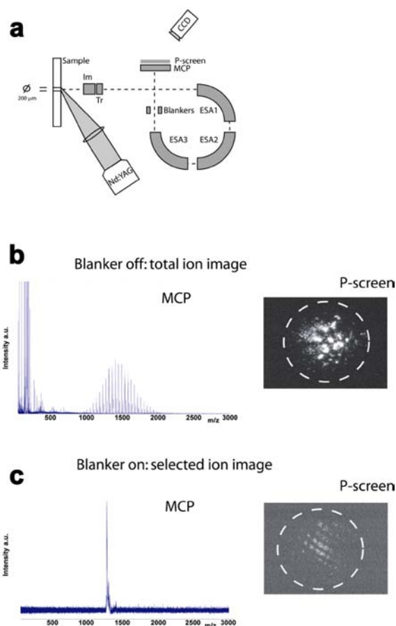
Figure 2. Instrumentation of the stigmatic mass microscope and a comparison with microprobe IMS. (A) Schematic representation of the Physical Electronics Trift II mass spectrometer (B) TIC and (C) SIC stigmatic ion imaging.
