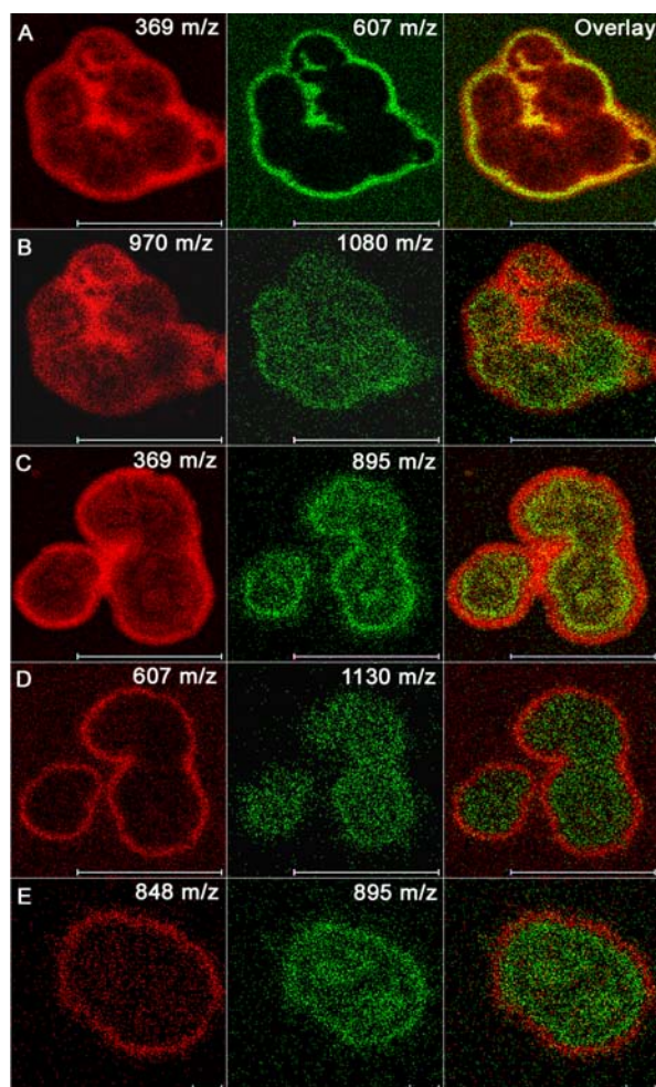
Figure 6. Cellular localization of MetA-SIMS selected ion count signals from neuroblastoma cells. Cells were imaged after deposition of 1-nm gold. (A) m/z 369 (cholesterol [M-OH]^+ , 0-14 counts) and m/z 607 (DAG, 0-6 counts). (B) m/z 970 (cholesterol [2M+Au]^+ , 0-4 counts) and m/z 1080 (0-1 counts). (C) m/z 369 (cholesterol [M-OH]^+ , 0-12 counts) and m/z 895 (0-2 counts). (D) m/z 607 (DAG, 0-4 counts) and m/z 1130 (0-1 counts). (E) m/z 848 (0-1 counts) and m/z 895 (0-1 counts). (Au)_n marks indicate the gold-cluster m/z values. Scale bar: 100 \mu m in panels A-D and 10 \mu m in panel E. Total ion dose 1.18 \times 10^{12} ions/cm 2 in panels A-D and 4.7 \times 10^{12} ions/cm 2 in panel E.
