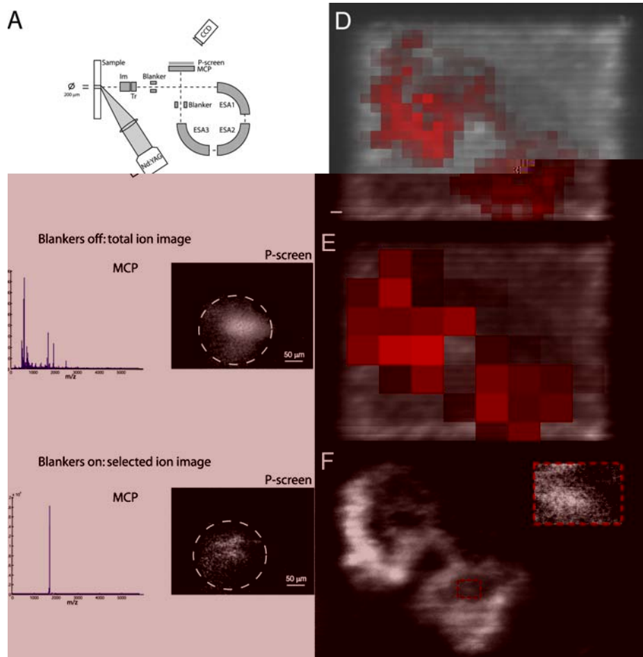
Figure 1. Instrumentation of the stigmatic mass microscope and a comparison with microprobe IMS. (A) Schematic representation of the Physical Electronics Trift II mass spectrometer (B) TIC and (C) stigmatic single ion imaging. The distribution of the neuropeptide \alpha -MSH (diacetylated) in microprobe imaging, depicted with a resampled pixel size of (D) 80×80 \mu\text{m} (red) and (E) 250×250 \mu\text{m} (red) and overlaid on the stigmatic TIC image, is compared to (F) the stigmatic ion image of diacetylated- \alpha -MSH, with in the inset an enlarged area of the ion distribution. Scale bar is 100 \mu\text{m} .
