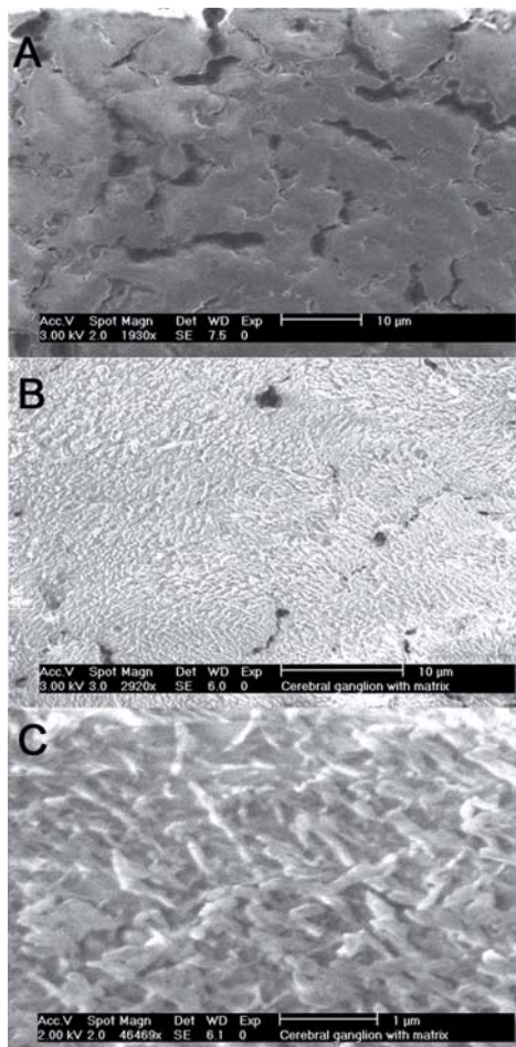
Figure 5. Scanning electron microscopy images of Lymnaea stagnalis nervous tissue (A) prior to matrix application (scale bar 10 \mu\text{m} ) and (B) after ESD of DHB (scale bar 10 \mu\text{m} ). (C) Higher magnification image showing sub-micron crystal dimensions after ESD (length \sim 0.5\text{-}1 \mu\text{m} , width \sim 0.2\text{-}0.4 \mu\text{m} ) (scale bar 1 \mu\text{m} ).
