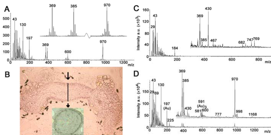
Figure 1. SIMS imaging of cholesterol and Lymnaea stagnalis nervous tissue with (A) MetA-SIMS spectrum of cholesterol spotted on a gold coated (5nm) silicon wafer (high mass range enhanced by factor of 2.5) (B) Optical microscopy image of Lymnaea stagnalis nervous tissue showing the left and right cerebral ganglia and the connecting commissure, inset shows cryomicrotome section of the commissure used in the MetA-SIMS analysis. (C) SIMS spectrum and (D) MetA-SIMS spectrum of Lymnaea stagnalis nervous tissue (high mass range enhanced by factor of 200 and 10 respectively).
