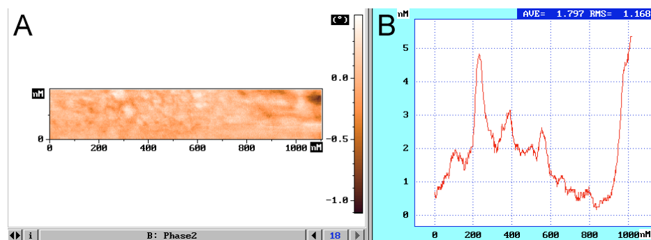
Figure 8. AFM measurement of gold nanoislands on top of a tissue section. A) AFM image of the tissue surface. B) plot of the width and height of the observed islands.
