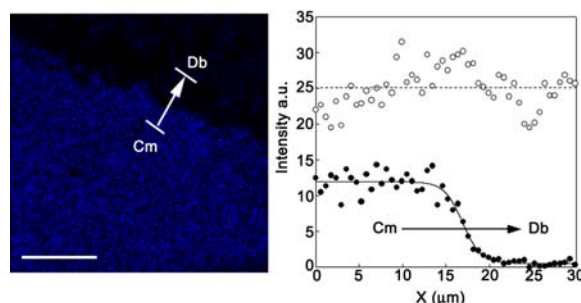
Figure 6. Experimental resolution of direct tissue ME-SIMS. (A) Cholesterol distribution (blue) in the commissure (Cm) and dorsal body (Db) area (dashed box in Figure 3C). Scale bar: 50 \mu\text{m} . The arrow indicates a line scan orthogonal to the commissure - dorsal body transition (length 30 \mu\text{m} , width 3.5 \mu\text{m} ). (B) Cholesterol (●) and DHB intensity data (○) of the same line scan.
