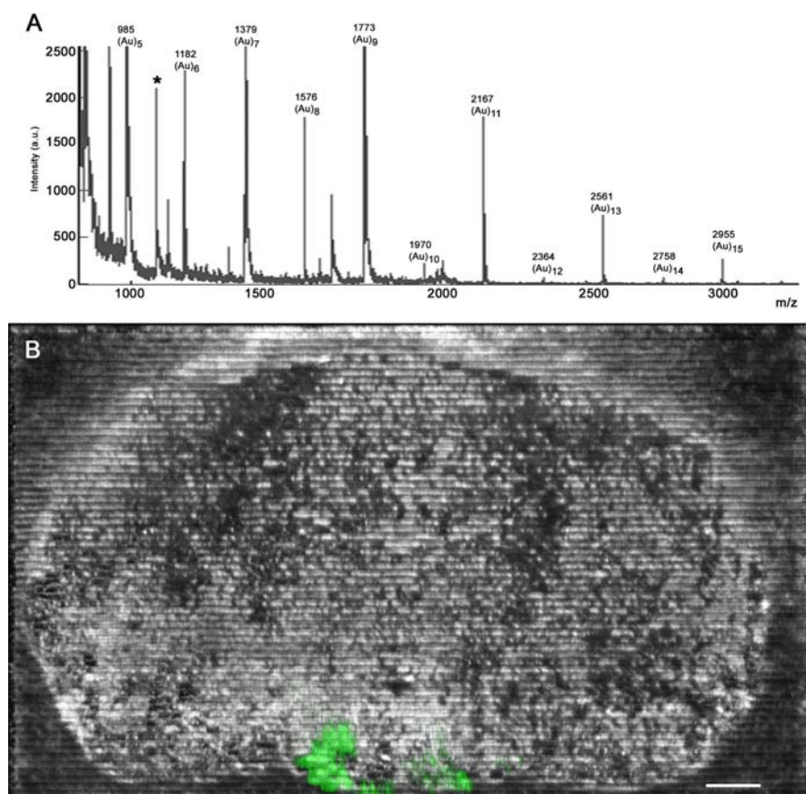
Figure 9. MALDI stigmatic imaging of a rat brain tissue section. (A) A line-scan summed mass spectrum showing gold cluster peaks and several peptide peaks, with the vasopressin mass at m/z 1085 (*). (B) The TIC image (gray-scale) of a 4-HCCA coated rat brain tissue section overlaid with the selected ion image for vasopressin (green). Scale bar: 1 mm.
