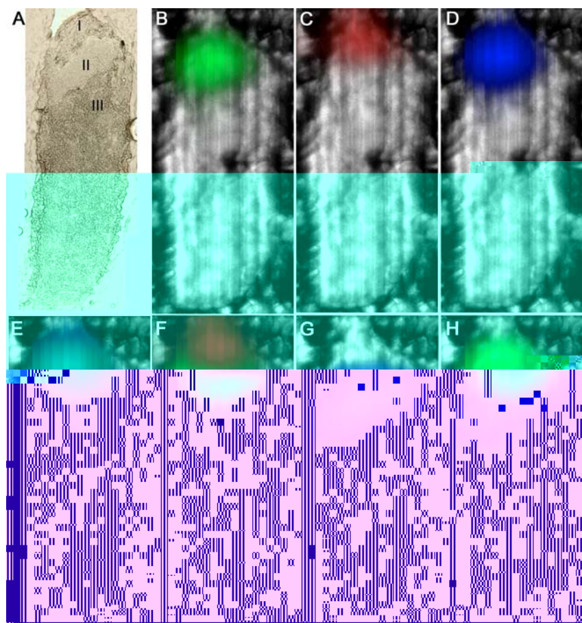
Figure 3. Molecular imaging of rat pituitary tissue by MALDI-IMS. (A) Optical image of an untreated rat pituitary tissue section, with (I) the posterior lobe, (II) the intermediate lobe and (III) the anterior lobe. (B) Distribution of the selected ion image of vasopressin (green), (C) oxytocin (red) and (D) c-terminal fragment of the ProVP precursor (blue) overlaid on the TIC image in grayscale. (E) Combined distributions of vasopressin (green) and the c-terminal fragment (blue) and (F) vasopressin (green) and oxytocin (red) overlaid on the TIC image in grayscale. (G) Distribution of the selected ion image of \alpha -MSH (blue) and (H) Combined distributions of vasopressin (green) \alpha -MSH (blue) overlaid on the TIC image in grayscale. Scale bar is 200 \mu m, tissue was covered with HCCA.
