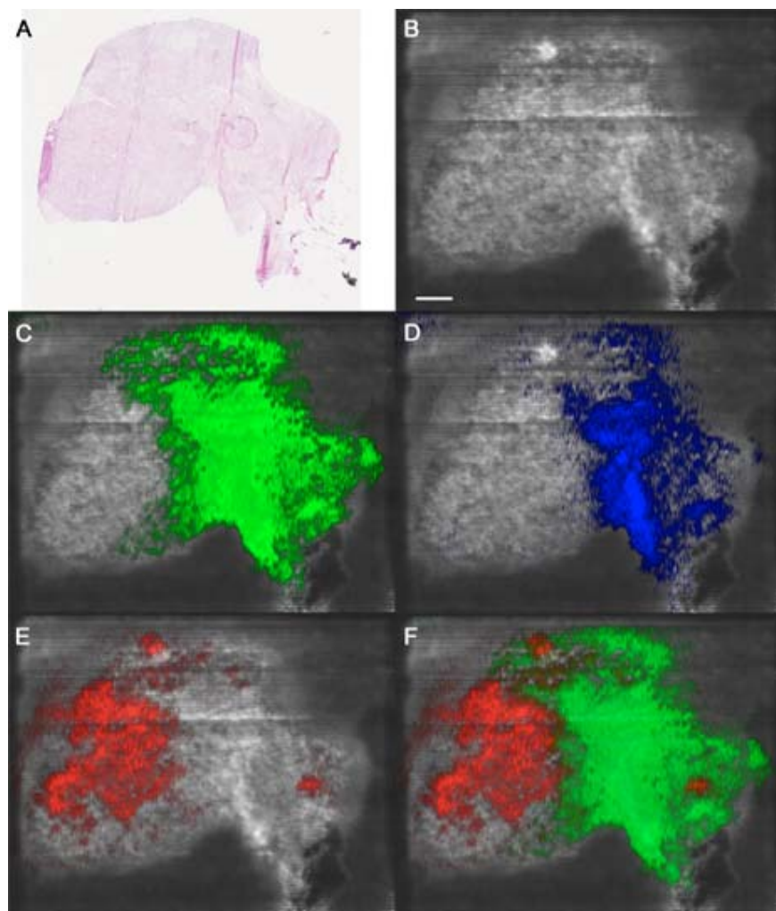
Figure 4. Molecular imaging of human pituitary tissue by MALDI-IMS. (A) Optical image of an H&E stained human pituitary tissue section. (B) TIC MALDI-IMS image in grayscale of a tissue section adjacent to the one in the optical image. Neuropeptide distributions overlaid on the grayscale TIC image with (C) vasopressin in green (D) oxytocin in blue (E) \alpha -MSH in red. (F) Overlay of vasopressin (green) and \alpha -MSH (red). Scale bar is 1 mm.
