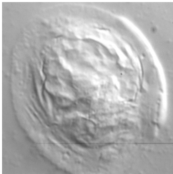
Figure 4. Differential interference contrast (DIC) microscope image of a single neuroblastoma cell after washing and drying. Field of view: 50×50 μm.
