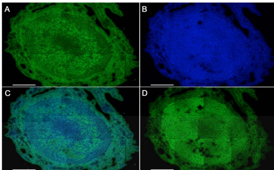
Figure 2. (A) MetA-SIMS image of cholesterol pseudomolecular ion [M-H]^+ distribution ( m/z 385, green, 0-20 counts). (B) MetA-SIMS image of cholesterol fragment ion [M-OH]^+ distribution ( m/z 369, blue, 0-16 counts). (C) Overlay image of cholesterol pseudomolecular ion [M-H]^+ ( m/z 385, green, 0-20 counts) and cholesterol fragment ion [M-OH]^+ distributions ( m/z 369, blue, 0-25 counts). (D) MetA-SIMS image of cholesterol pseudomolecular ion distribution [2M+Au]^+ ( m/z 970, green, 0-5 counts). Scale bars are 100 \mu m .
