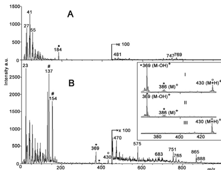
Figure 4. ToF-SIMS spectra of the Lymnaea nervous tissue before (A) and after (B) ESD matrix deposition. Marked peaks are: DHB ( M ) + at 154 m/z and ( M -OH) + at 137 m/z (#), phosphocholine fragment ion at 184 m/z (•), cholesterol ( M ) + at 386 m/z and ( M -OH) + at 369 m/z (*), and APGWamide ( M +H) + at 430 m/z (◊). Inset shows (I) zoomed area of spectrum B and ME-SIMS spectra of (II) synthetic cholesterol and (III) synthetic APGWamide.
