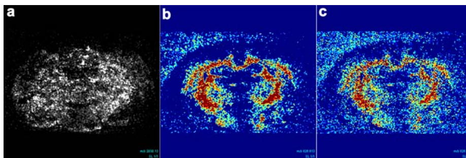
Figure 5. Example of images obtained with microprobe MALDI-IMS on an Applied Biosystems 4700 proteomics analyzer and processed with BioMap software. (a) Distribution of a selected mass (m/z 2030) in grayscale and (b) of a selected mass (m/z 826.6) in color scale (Split-blue-red). (c) Same image as in panel b but now without interpolation.
