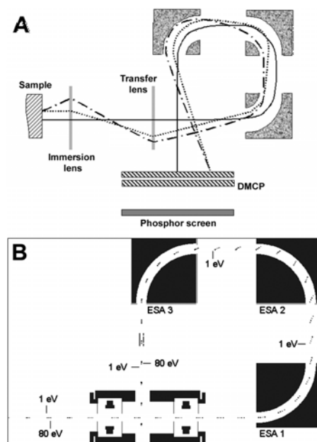
Figure 4. Schematic representation of the TRIFT ion microscope.
