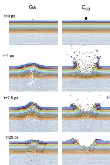
Figure 1. Cross-sectional view of the temporal evolution of a typical collision event leading to ejection of atoms due to 15 keV Ga^+ and C_{60}^+ bombardment of a silver metal surface at normal incidence. The atoms are colored by original layers in the substrate. The projectile atoms are black. (Taken from ref. 97 )
